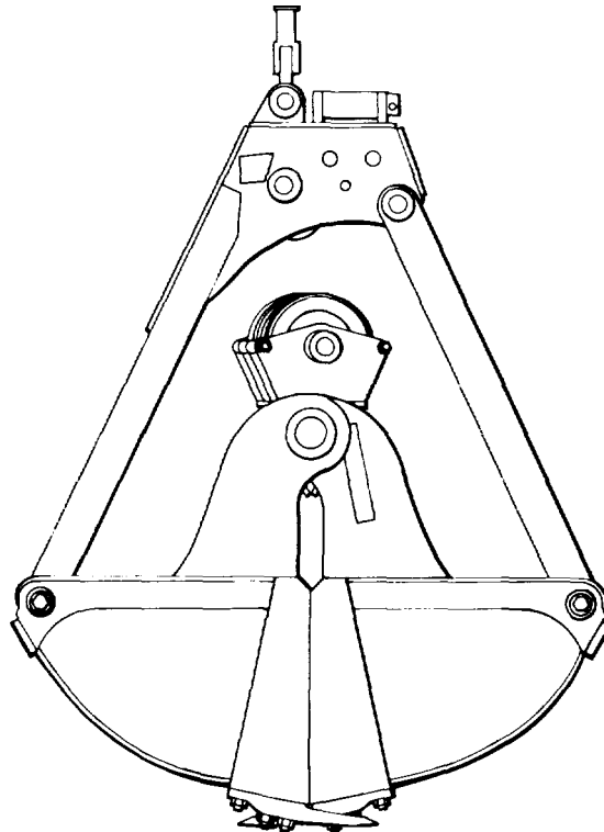
BUCKET, CLAMSHELL, TYPE II SIZE 75 3/4 CU. YD. GENERAL PURPOSE INTERGY MODEL 34GP S NSN 3815-01-249-4092
